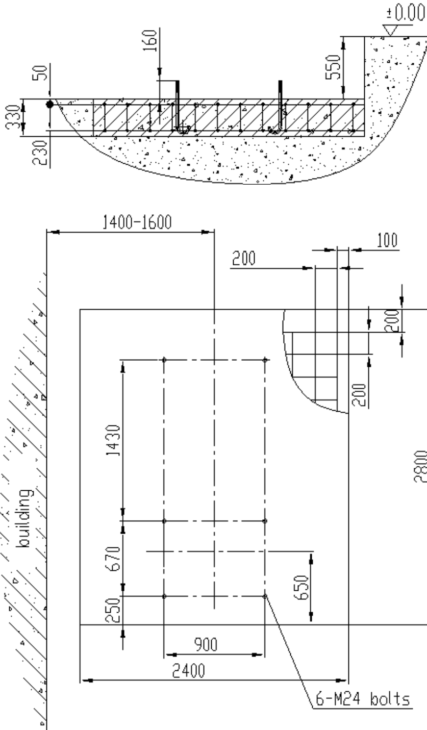
Hoist foundation
